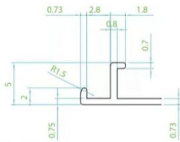
DETAIL "A" SCALE 3/1
